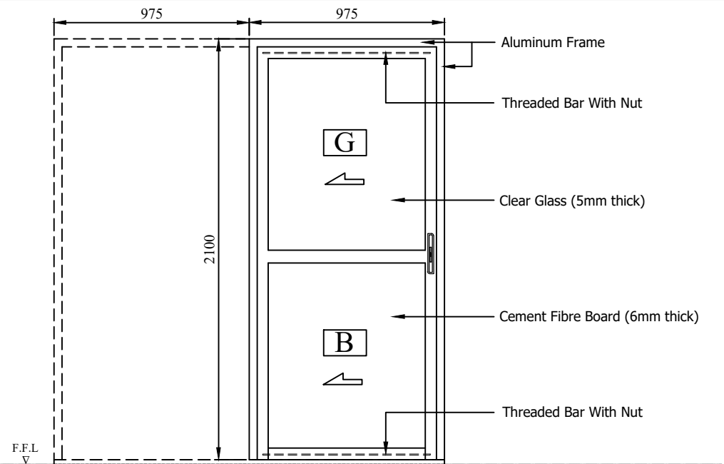
D26 - (GLAZED & BOARD SLIDING DOOR)
