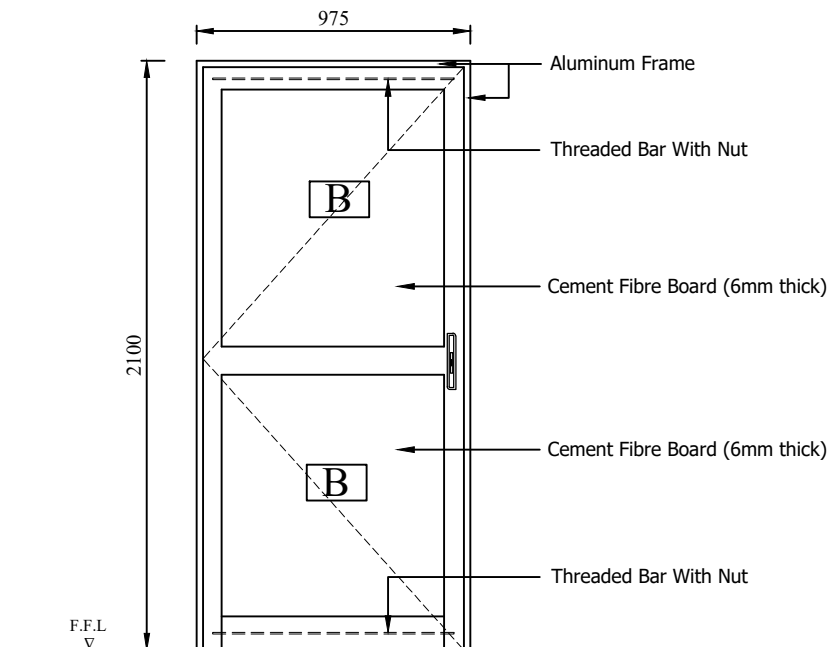
D27 - (FULL BOARD OPENABLE DOOR)
