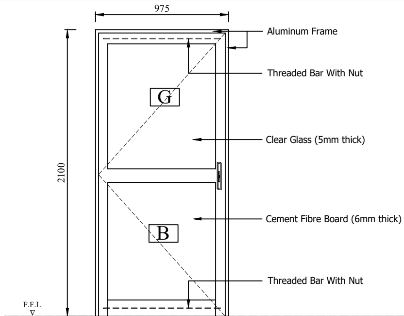
D25 - (GLAZED & BOARD OPENABLE DOOR)
