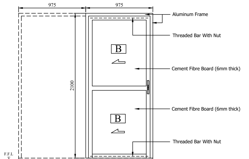
D28 - (FULL BOARD SLIDING DOOR)
