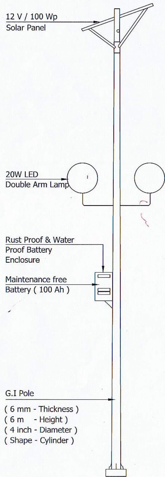
LAMP POST ( V - 225 )
