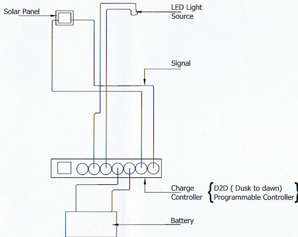
CIRCUIT DIAGRAM
